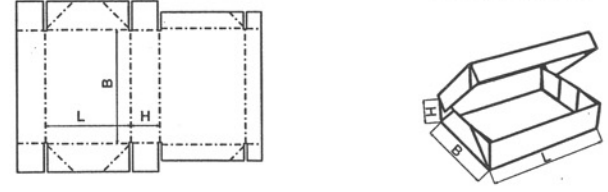
FEFCO 0770
