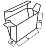
FEFCO 0445
