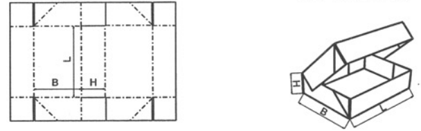
FEFCO 0760
