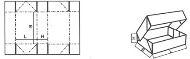
FEFCO 0761
