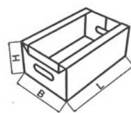
FEFCO 0440
