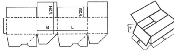
FEFCO 0713
