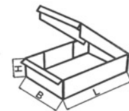
FEFCO 0441
