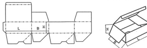
FEFCO 0714
