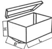
FEFCO 0313
