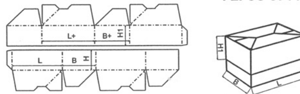
FEFCO 0714
