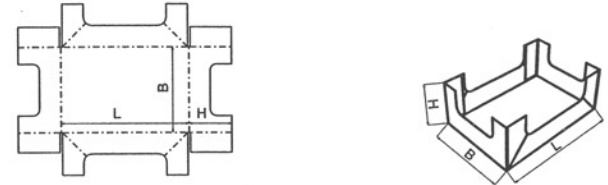
FEFCO 0770
